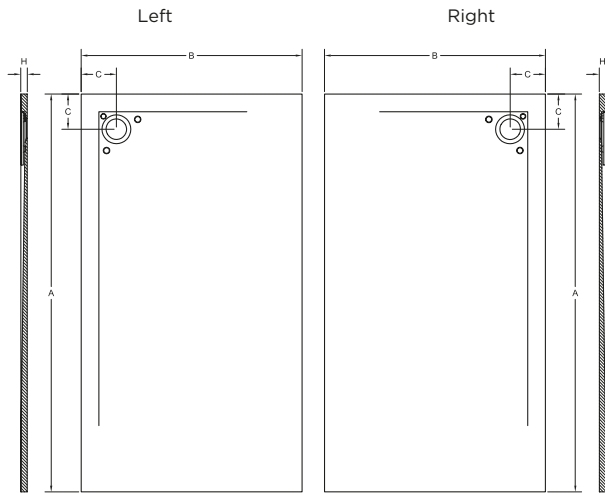
3.5" drain opening pre-drilled
